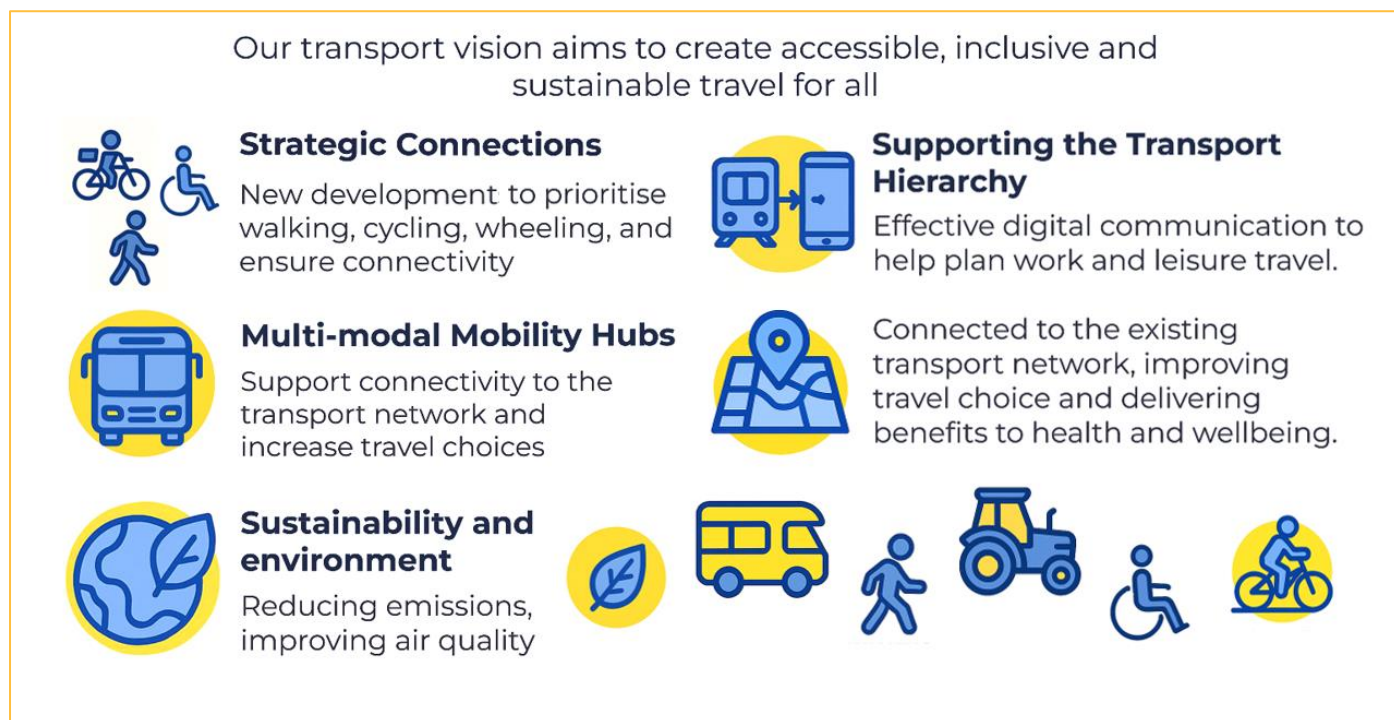
Figure 15 – Moving Torbay
